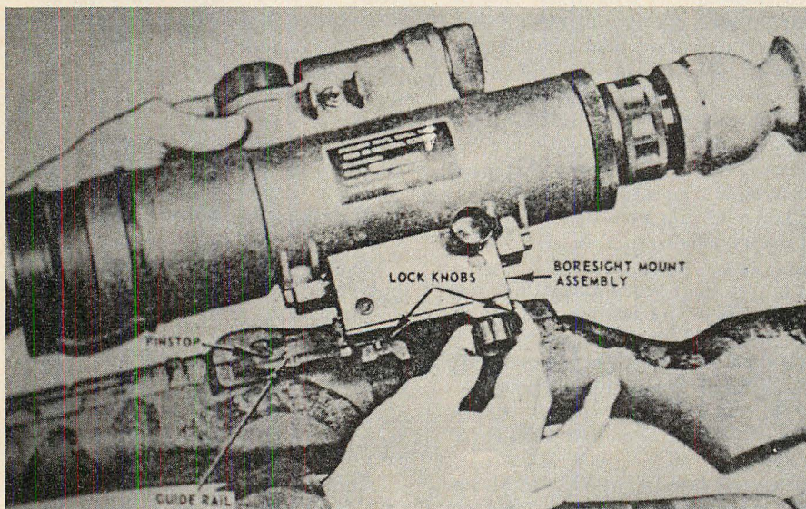
Nomenclature diagram of AN/PVS-2 Starlight (U.S. Army version) mounted on M-21 sniper rifle.
